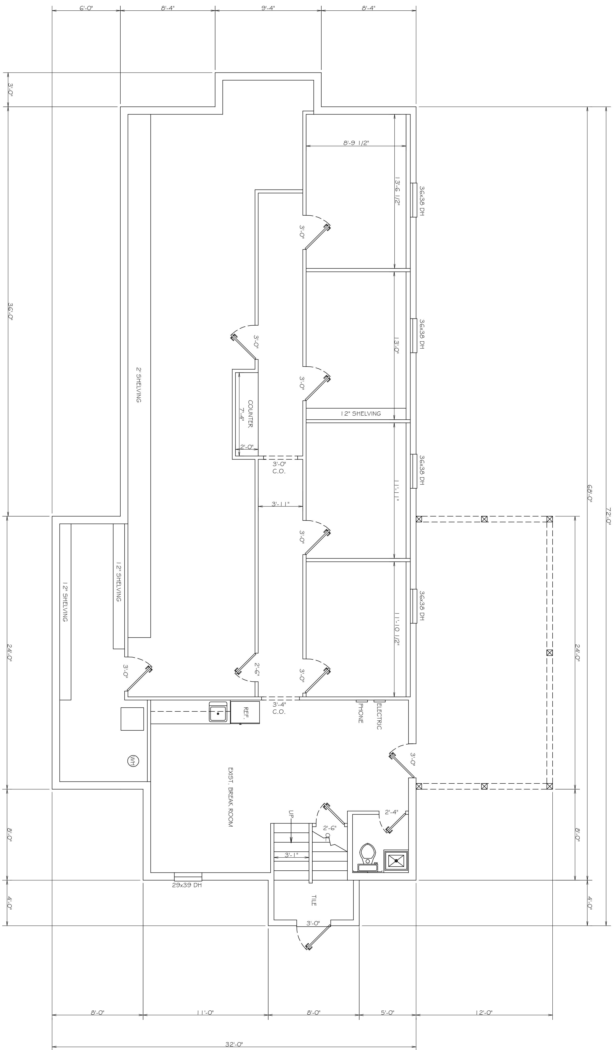
EXISTING LOWER FLOOR PLAN SCALE 1/4" = 1'-0"
